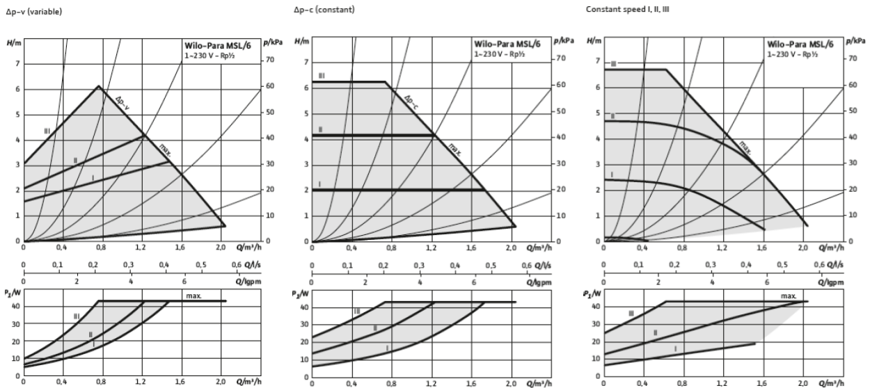
Abbildung 12: Pumpenkennlinien Figure 12: Characteristics of the circulating pump Figure 12: La caractéristique de la pompe de circulation
