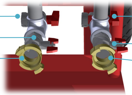
Figure 4: Connection assembly
